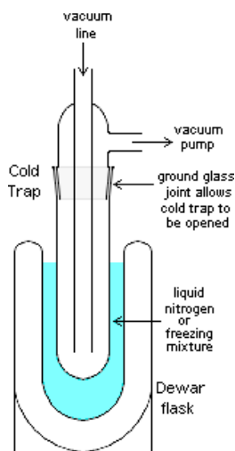
Figure 1: Cold Trap
